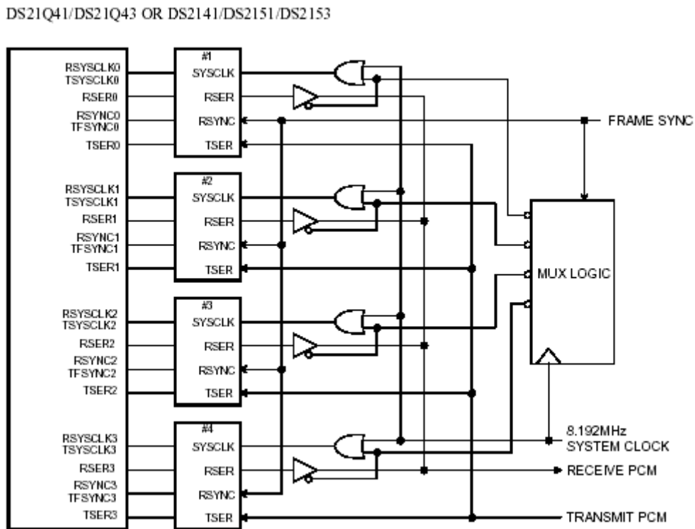
Figure 1. Quad Multiplexed Frames
